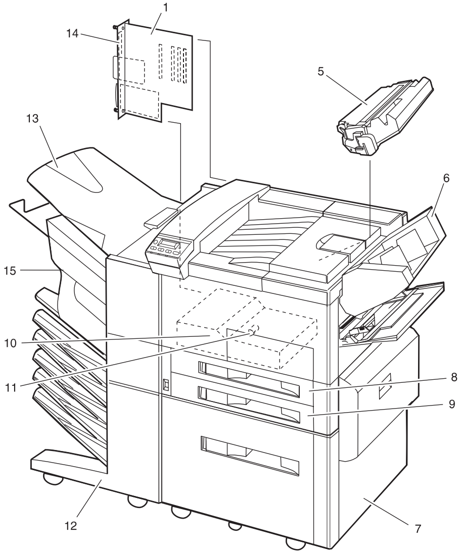
Figure 8-1 HP LaserJet 8000/N/DN or HP Mopier 240 Printer and Paper-Handling Components
