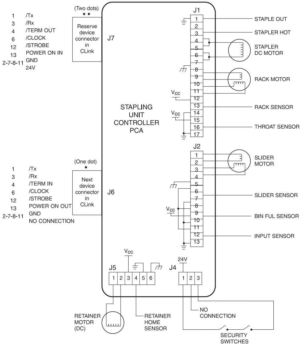
Figure 7-21 Mailbox with Stapler Wiring Diagram
