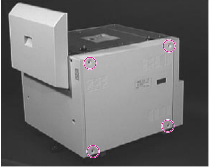
Figure 6-126 Back Cover
