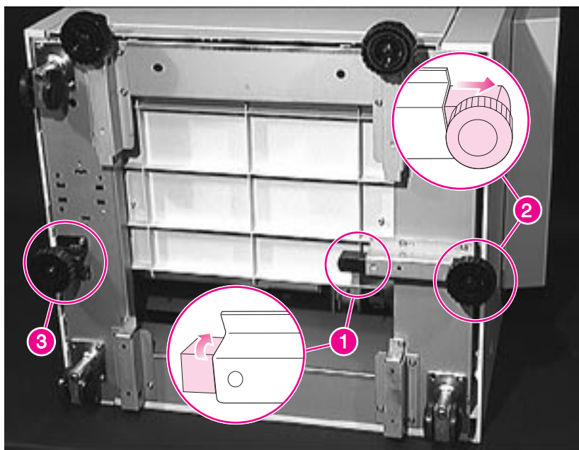
Figure 6-154 Foot Tip and Adjustable Foot Tip
