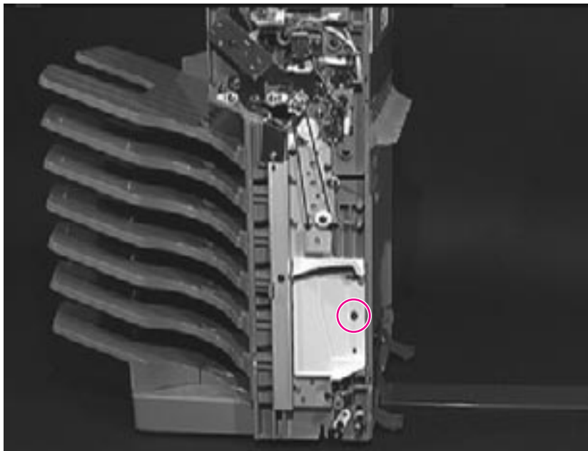
Figure 6-124 Cover Latch
