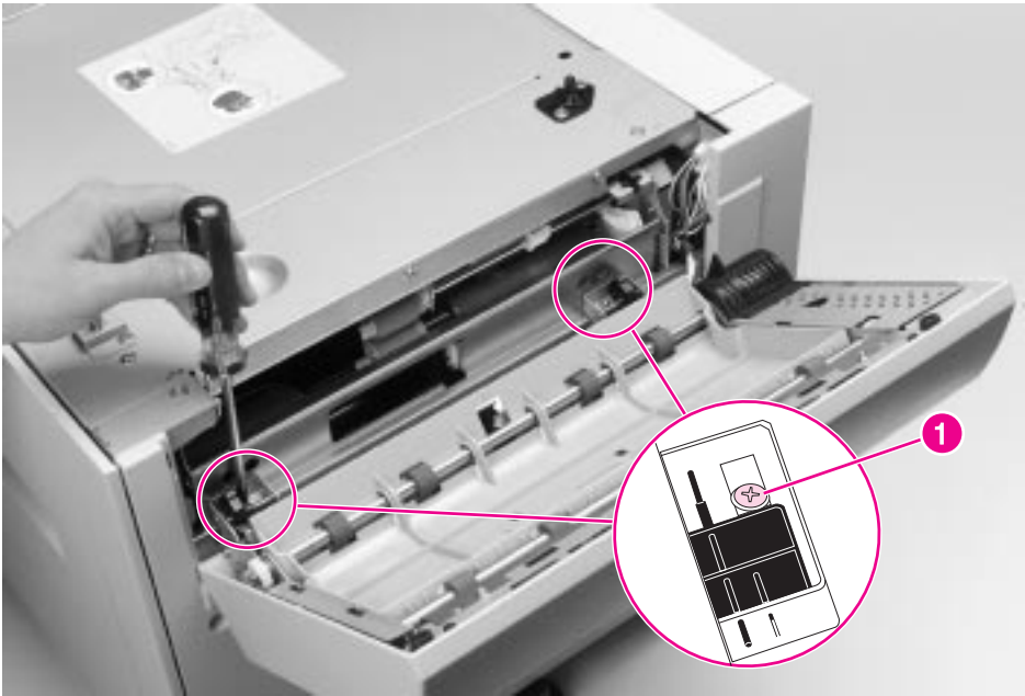
Figure 6-129 Vertical Transfer Unit (VTU) (2 of 3)
